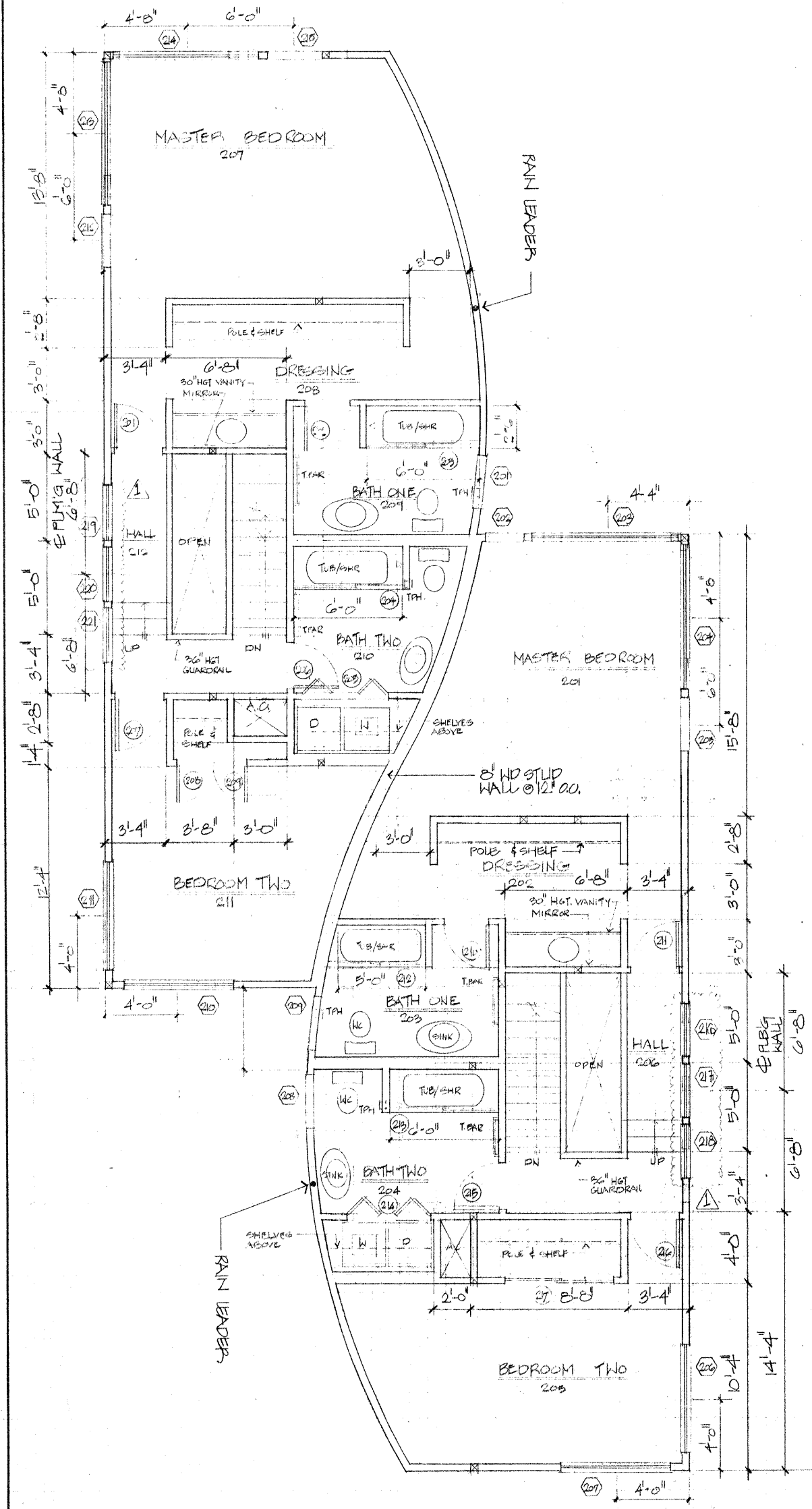
SECOND LEVEL PLAN NORTHEAST UNIT SW UNIT = 861# NE UNIT = 832# SCALE: 1/4" = 1'-0"
